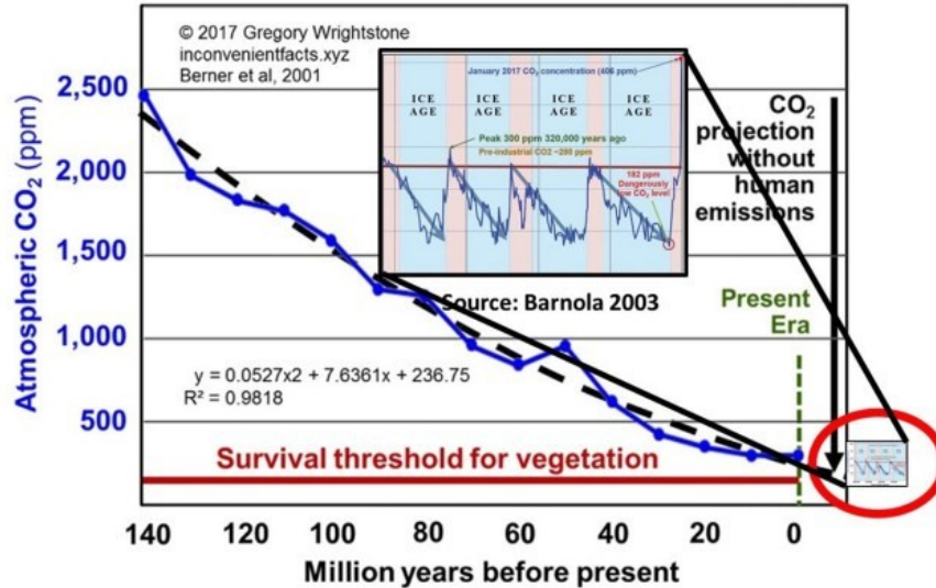
140 Million Years of Dangerous Decline in CO2
