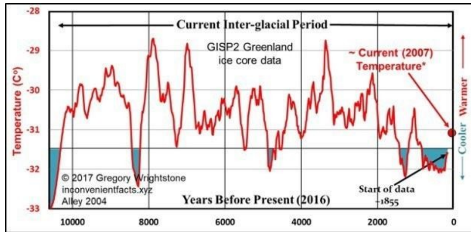
10,000 Years of Temperature
